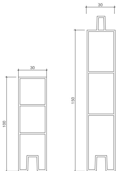
멀티엣지(W30) 알루미늄구조도(H100,150) SCALE : A1=1/1, A3=1/2
