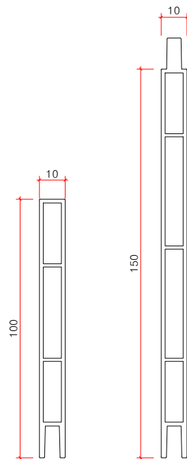
멀티엣지(W10) 알루미늄구조도(H100,150) SCALE : A1=1/1, A3=1/2
