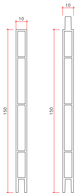
멀티엣지(W10) 알루미늄구조도(H150) SCALE : A1=1/1, A3=1/2
